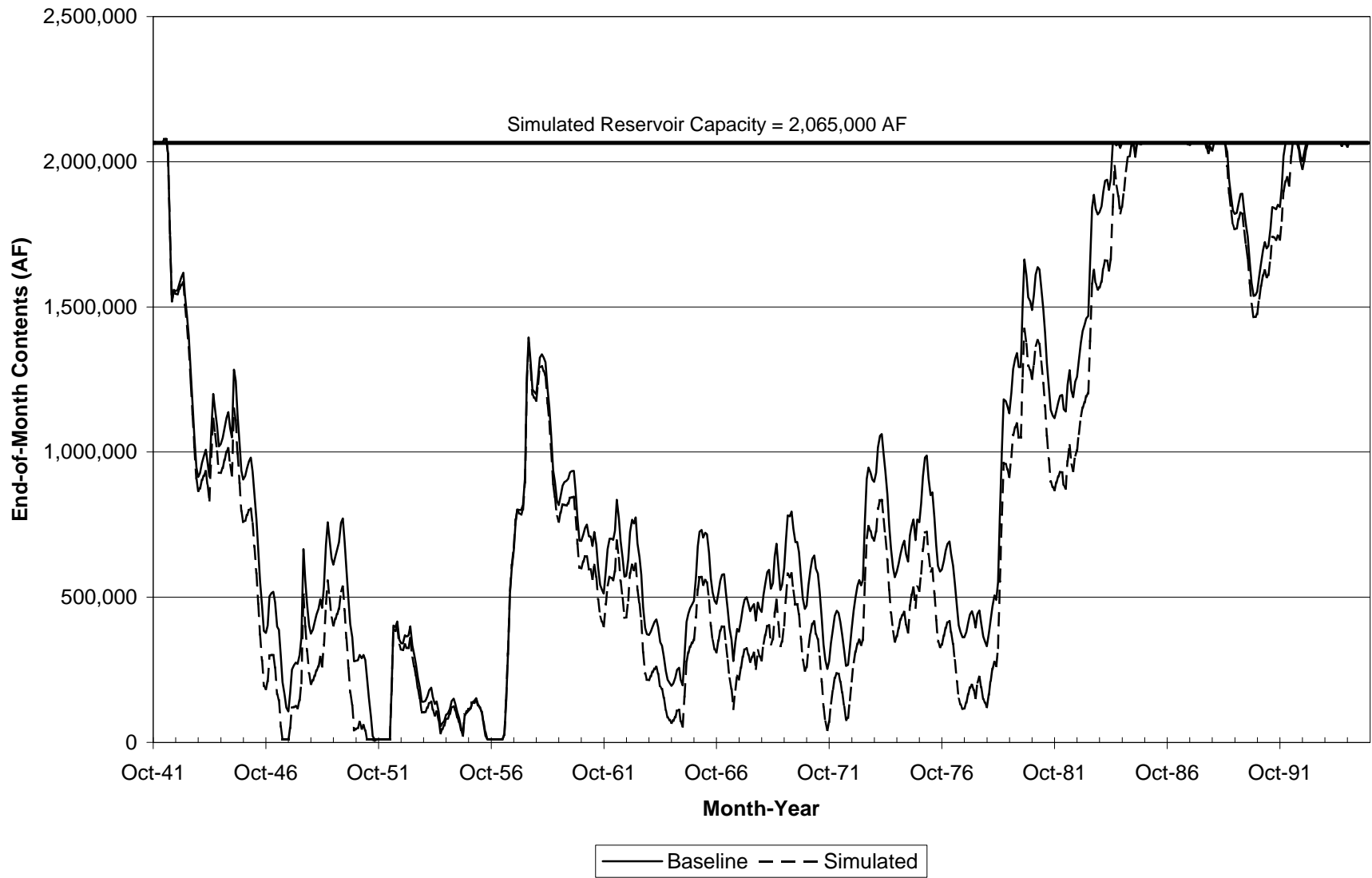
Figure 6.9 Alternatives A/B, Year 2010, Elephant Butte Reservoir - Simulated versus Baseline End-of-Month Contents
