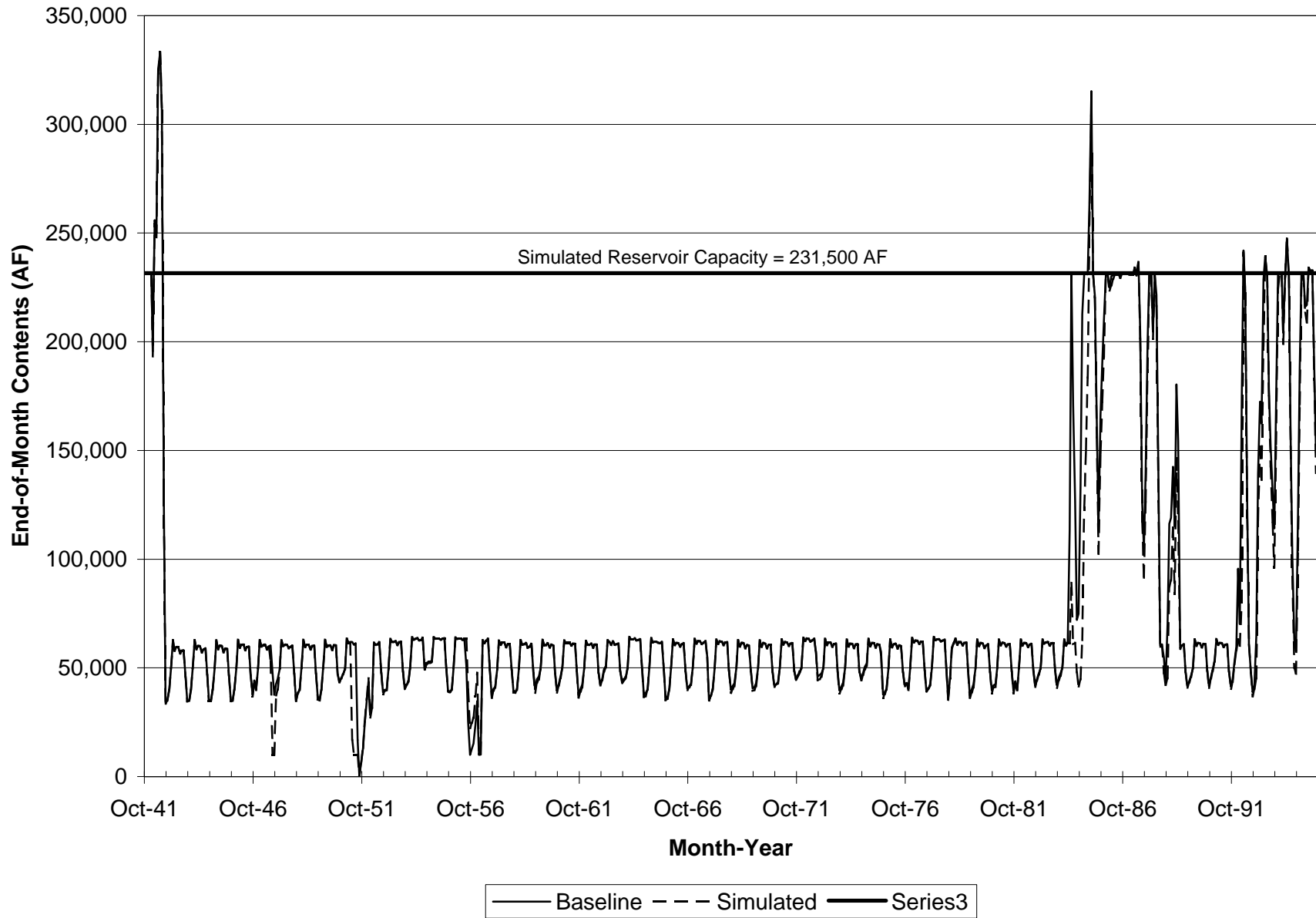
Figure 6.52 No Action Alternative, Year 2030, Caballo Reservoir - Simulated versus Baseline End-of-Month Contents
