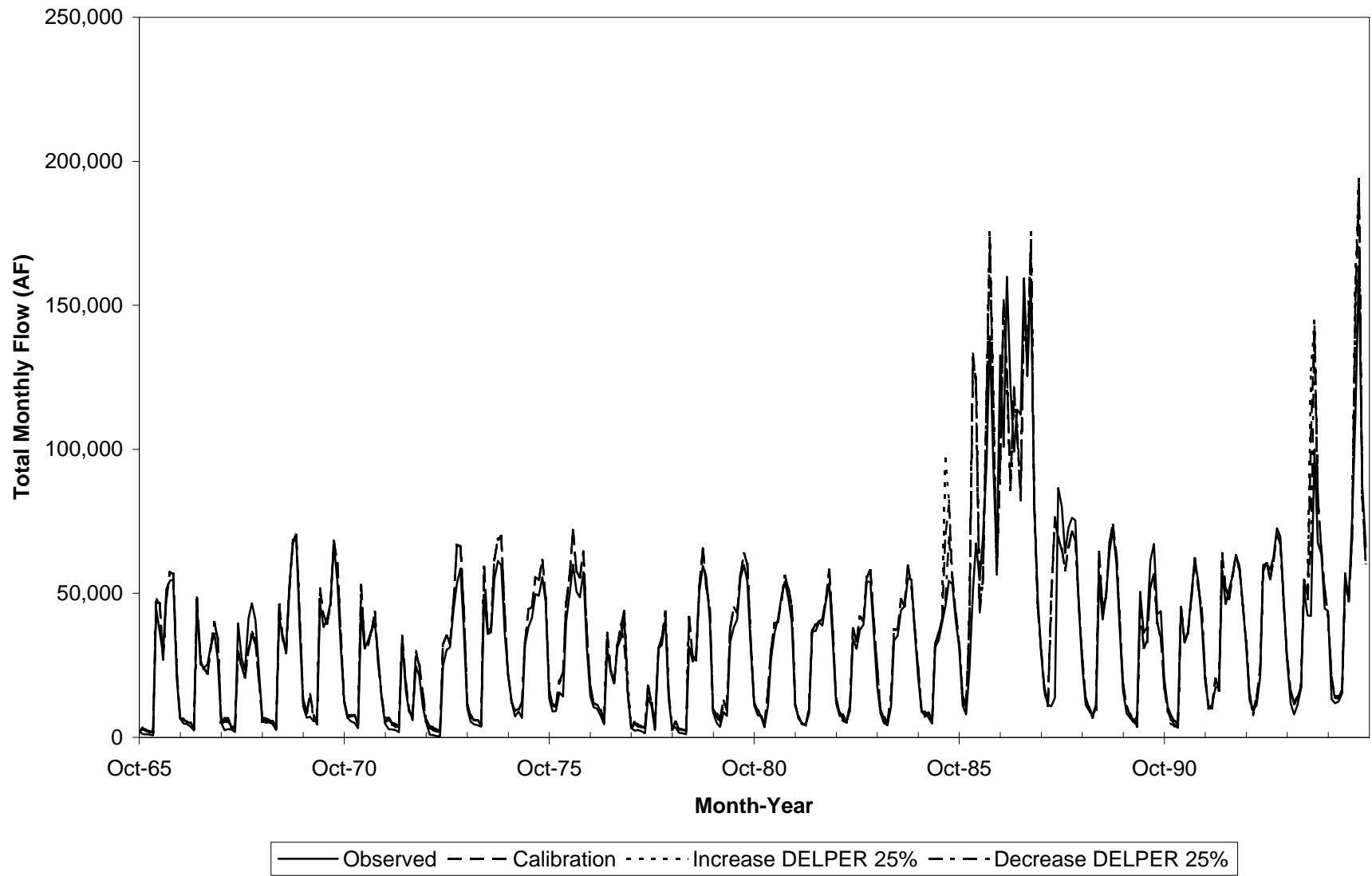
Figure 5.12 Mesilla Basin Delivery Efficiencies - Time Series Simulated versus Observed Flow at Rio Grande at El Paso
