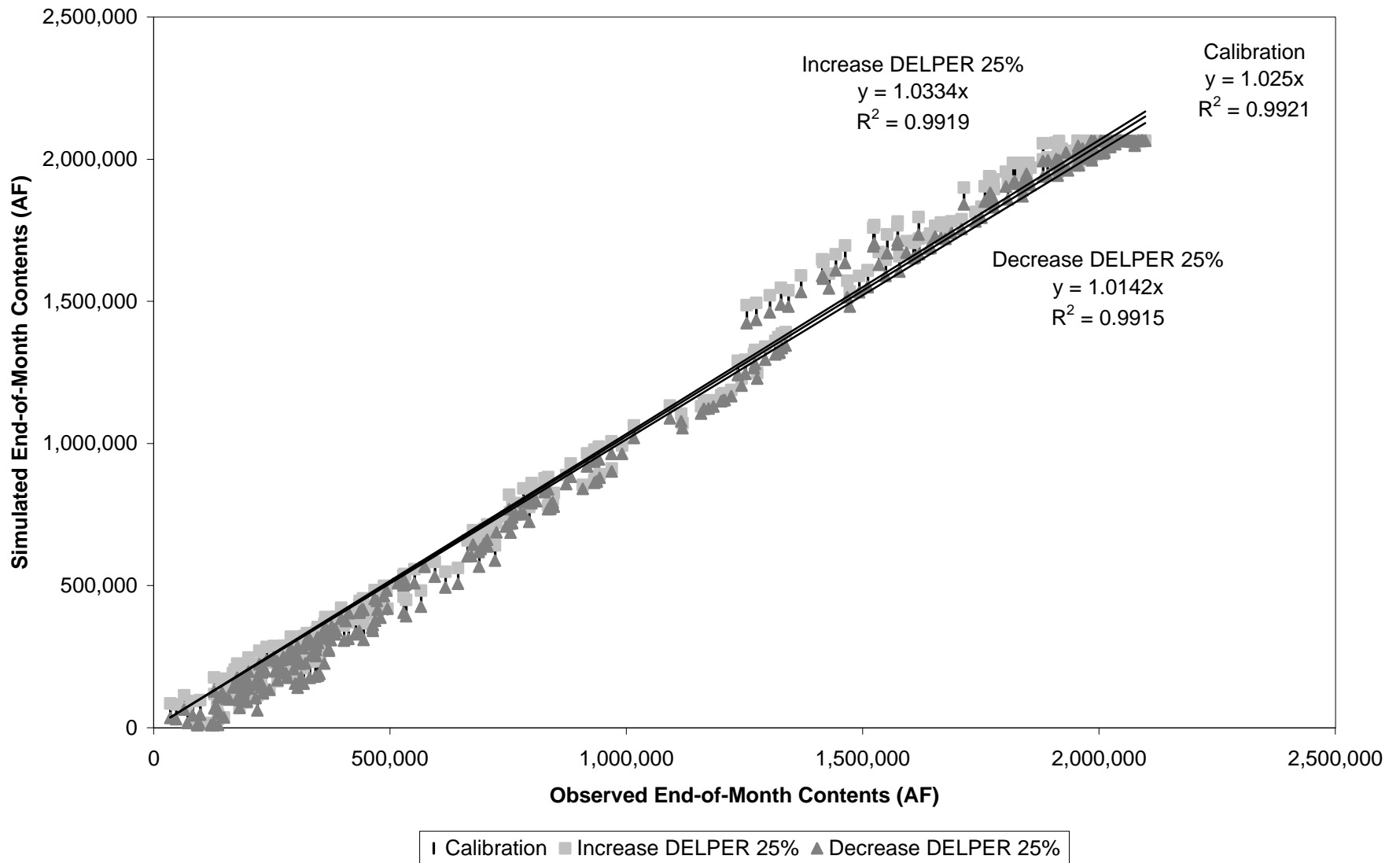
Figure 5.9 Mesilla Basin Delivery Efficiencies - Simulated versus Observed Elephant Butte Reservoir End-of-Month Contents
