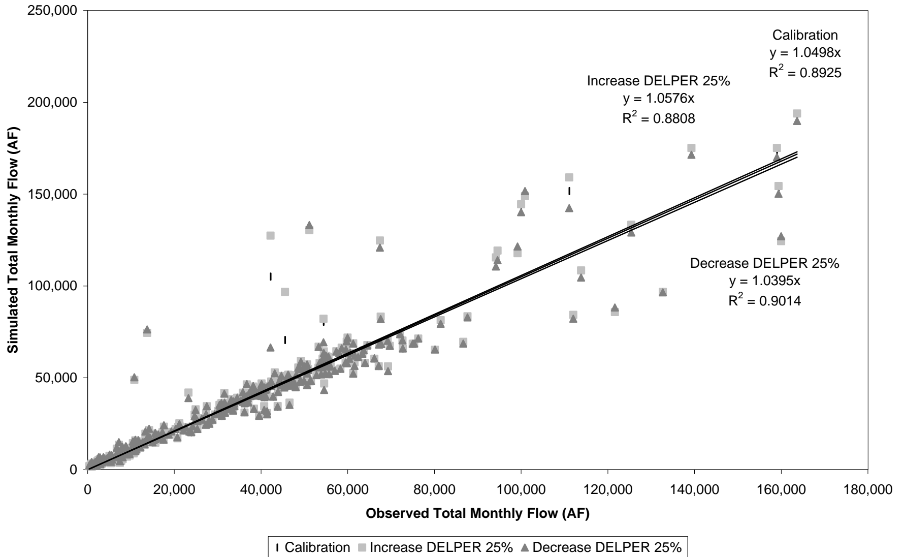
Figure 5.10 Mesilla Basin Delivery Efficiencies - Simulated versus Observed Flows at Rio Grande at El Paso
