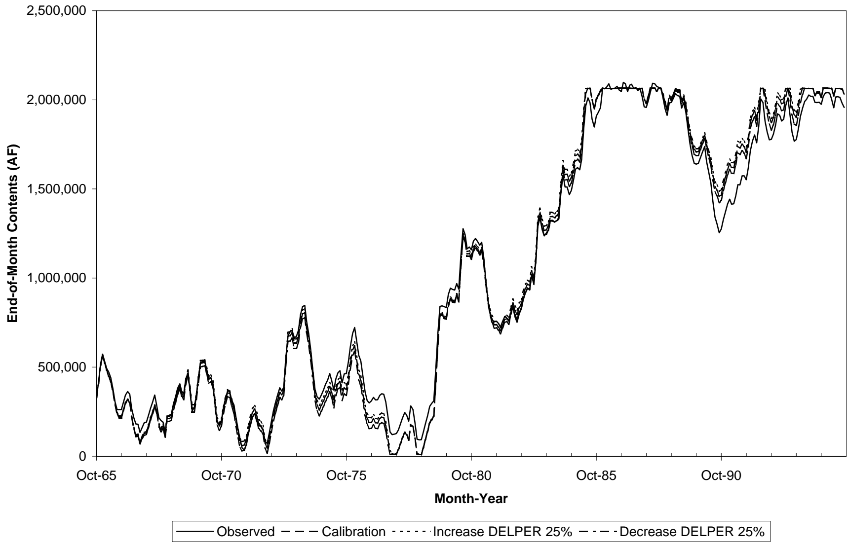
Figure 5.11 Mesilla Basin Delivery Efficiencies - Time Series Simulated versus Observed Elephant Butte Reservoir End-of-Month Contents
