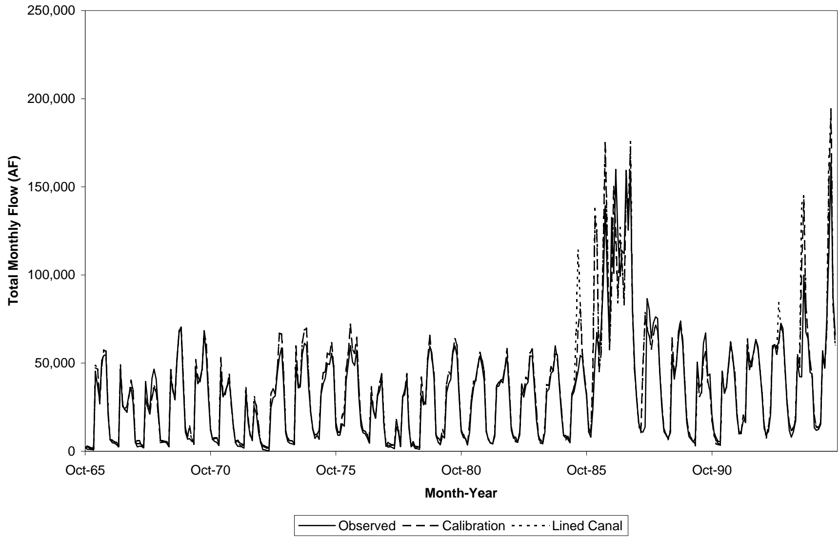
Figure 5.23 Canal Seepage - Time Series Simulated versus Observed Flows at Rio Grande at El Paso
