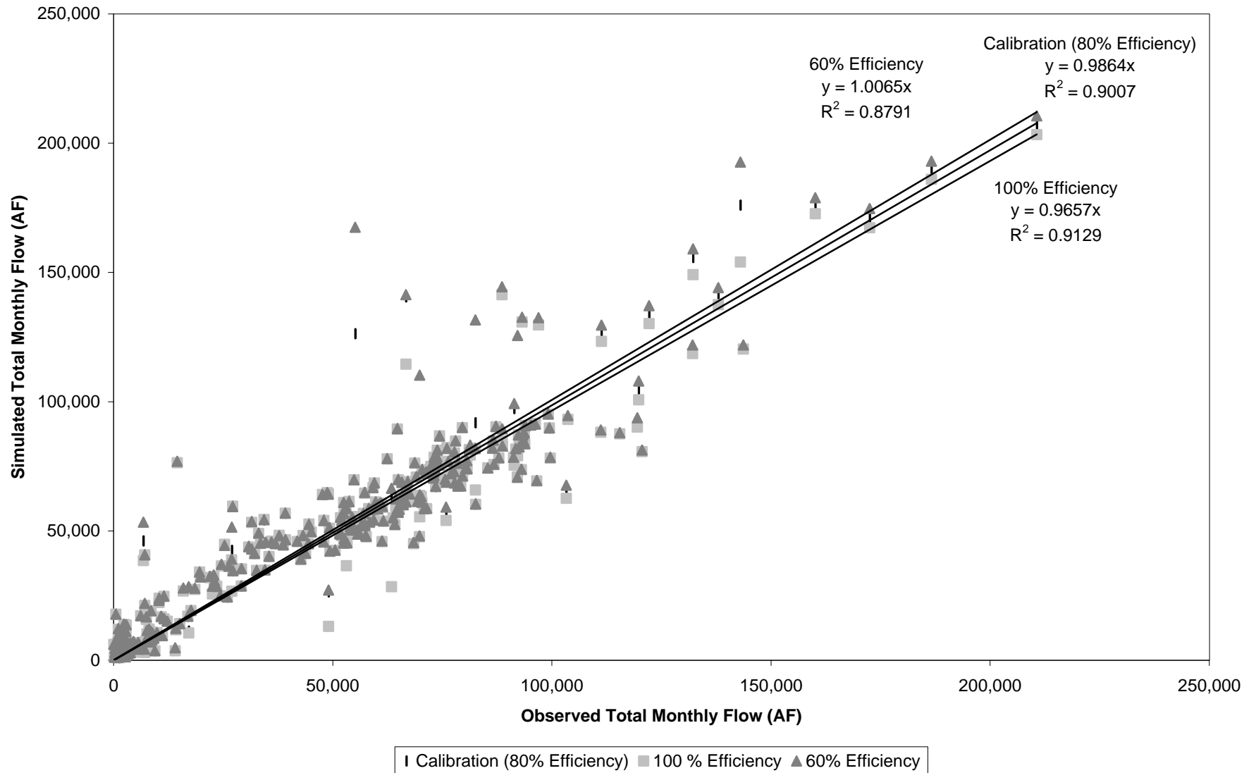
Figure 5.2 Rincon Irrigation Efficiencies - Observed versus Simulated Flow at Rio Grande below Leasburg Diversion Dam
