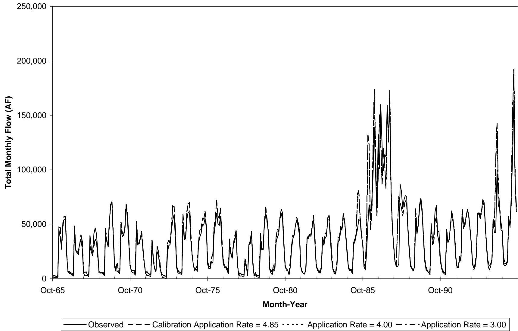
Figure 5.19 Pumping Demands - Time Series Simulated versus Observed Flow at Rio Grande at El Paso
