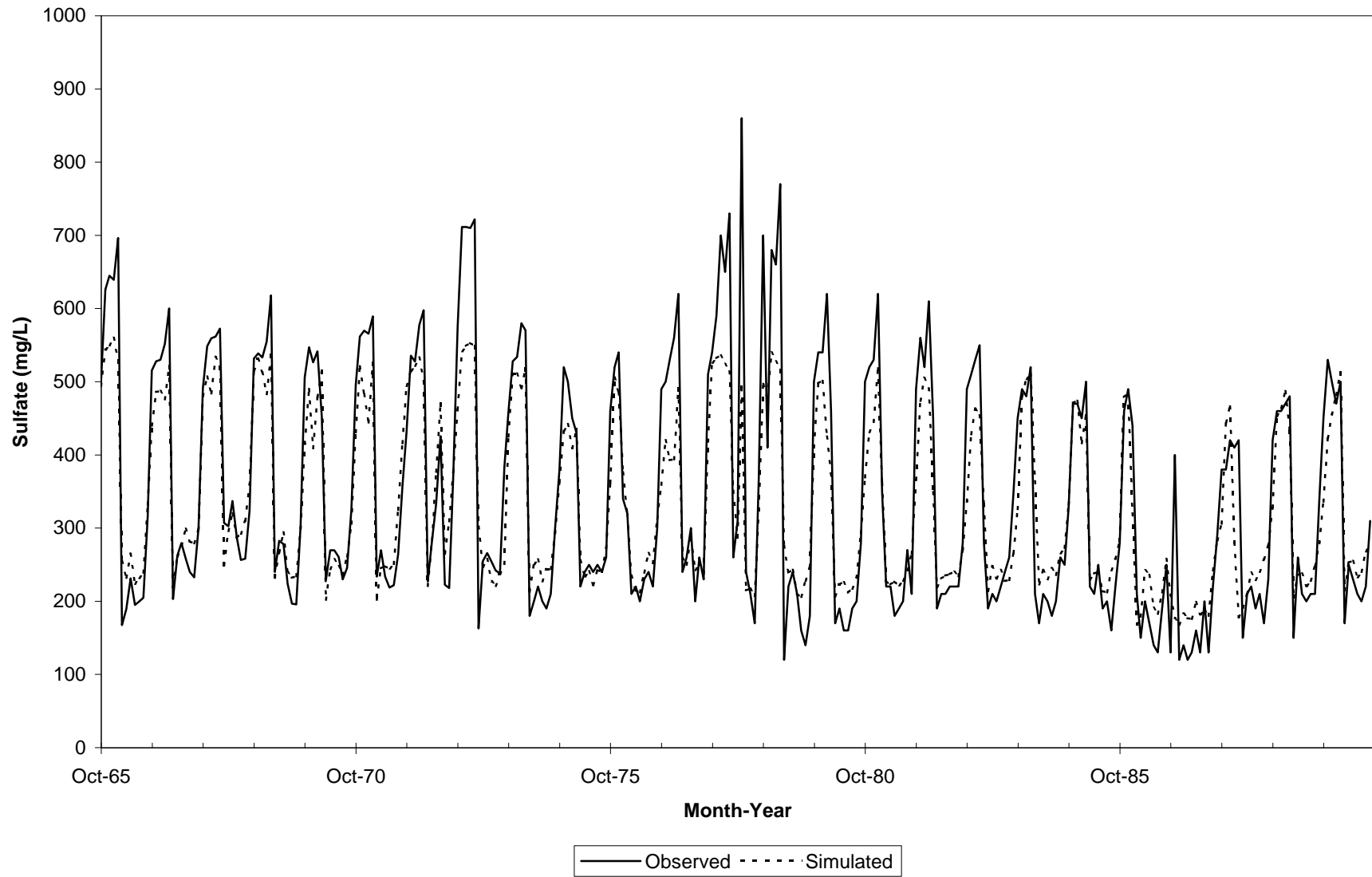
Figure 4.30 Rio Grande at El Paso - Simulated versus Observed Sulfate
