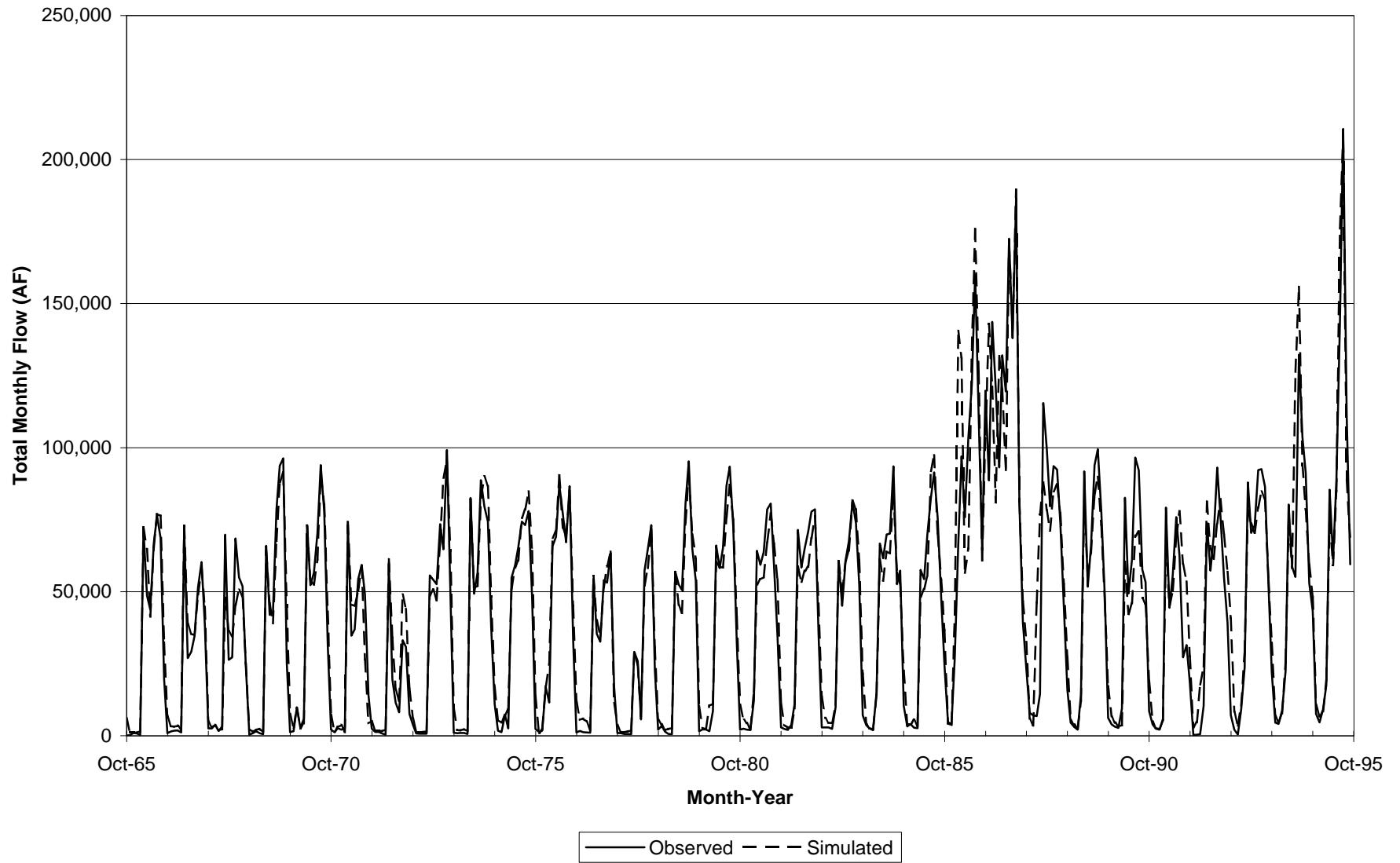
Figure 4.3 Rio Grande below Leasburg Diversion Dam - Simulated versus Observed Monthly Flow
