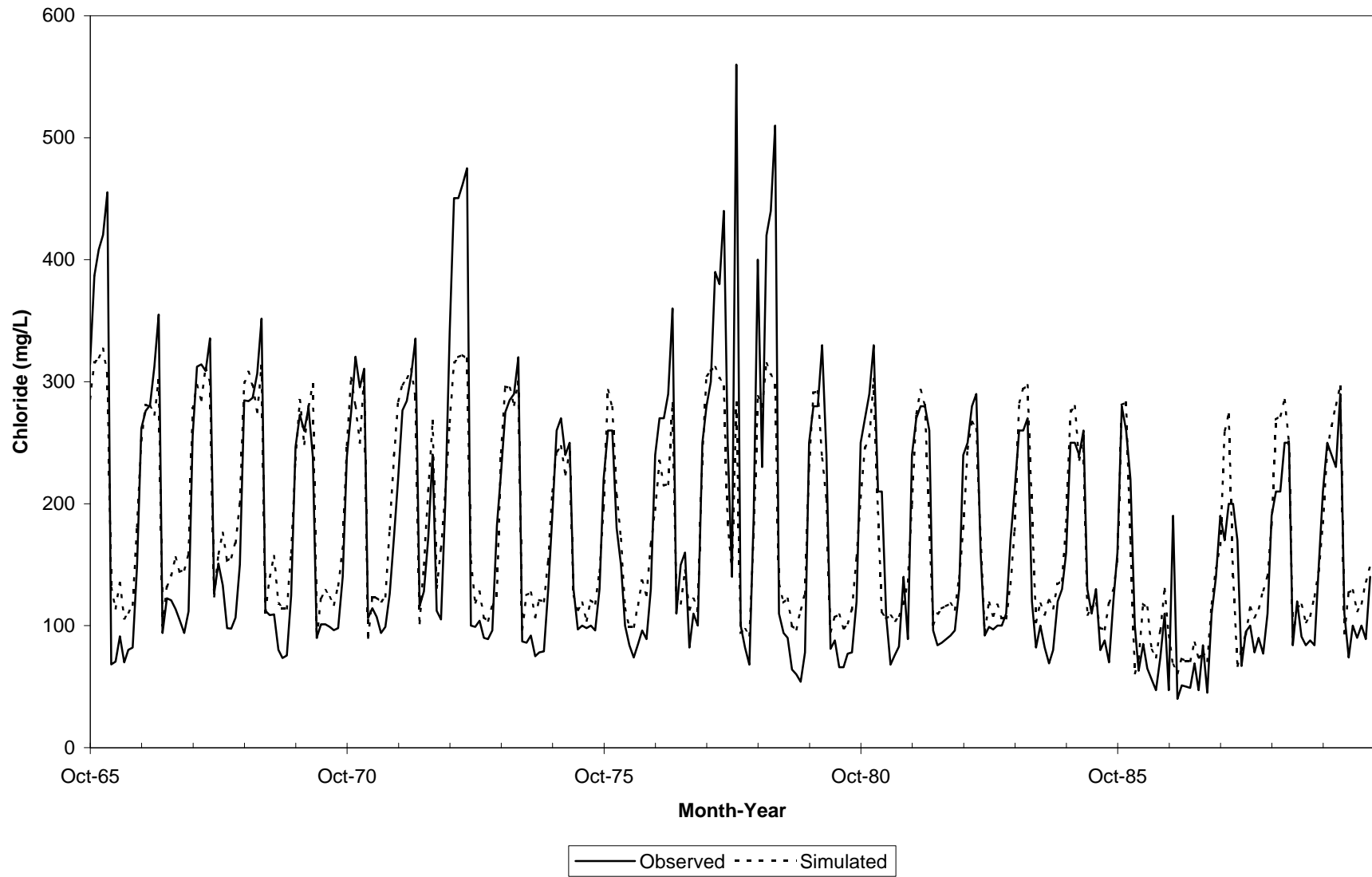
Figure 4.29 Rio Grande at El Paso - Simulated versus Observed Chloride
