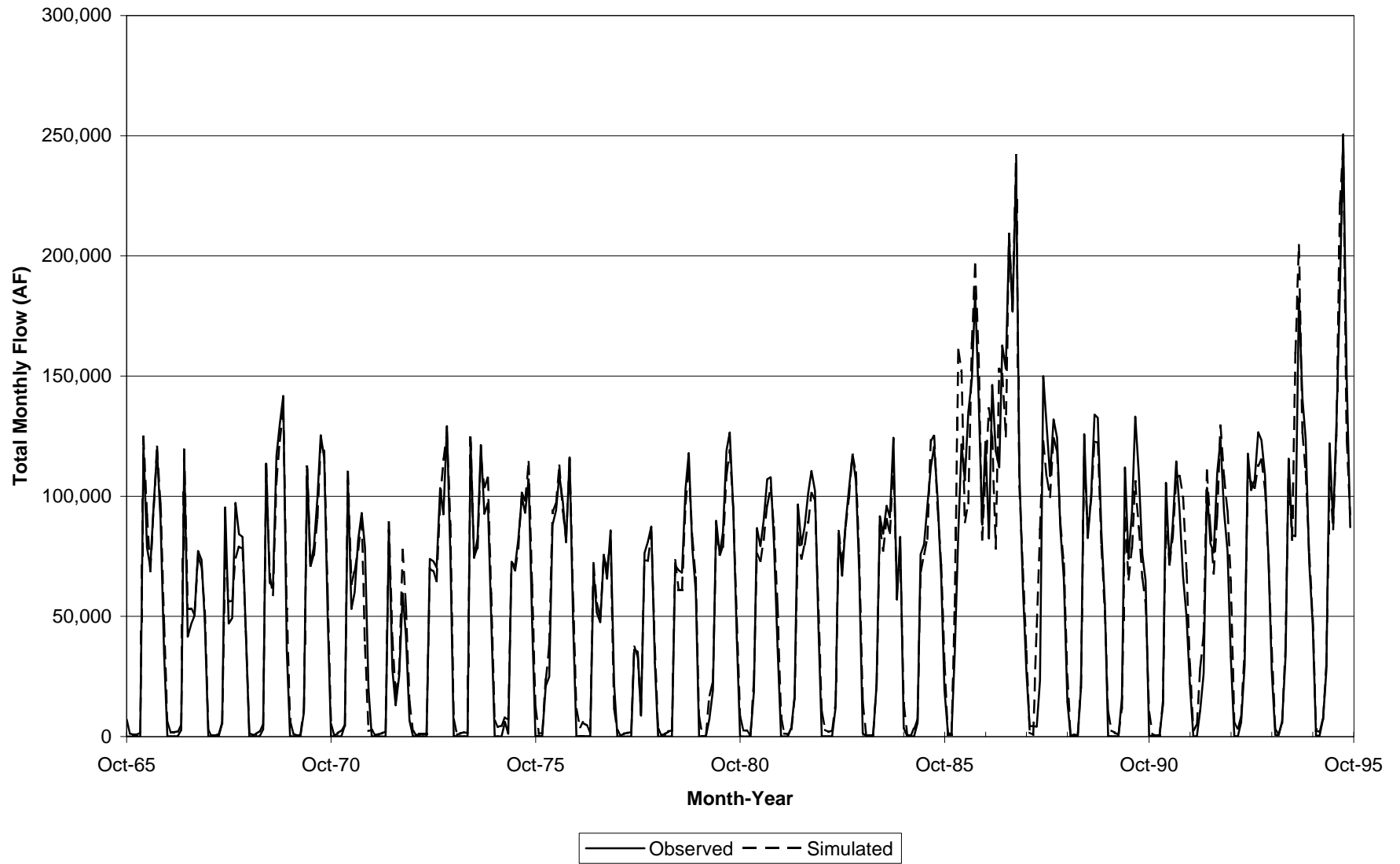
Figure 4.2 Rio Grande below Caballo Reservoir - Simulated versus Observed Monthly Flow
