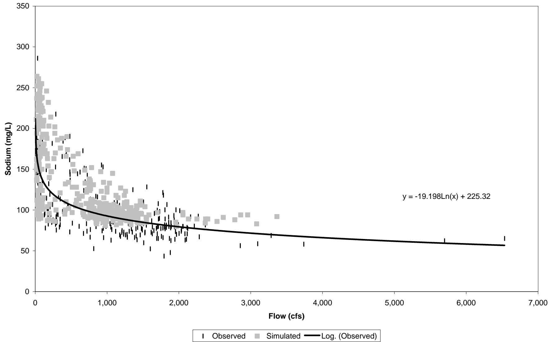
Figure 4.19 Rio Grande below Leasburg Diversion Dam - Sodium versus Flow
