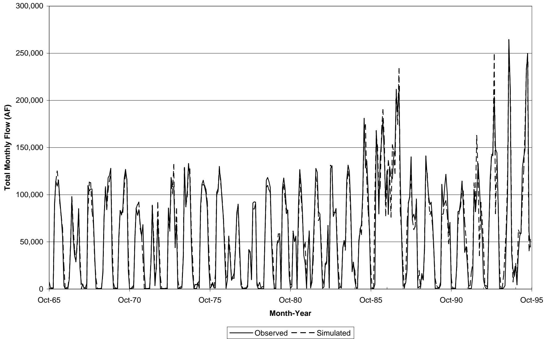
Figure 4.1 Rio Grande below Elephant Butte Reservoir - Simulated versus Observed Monthly Flow
